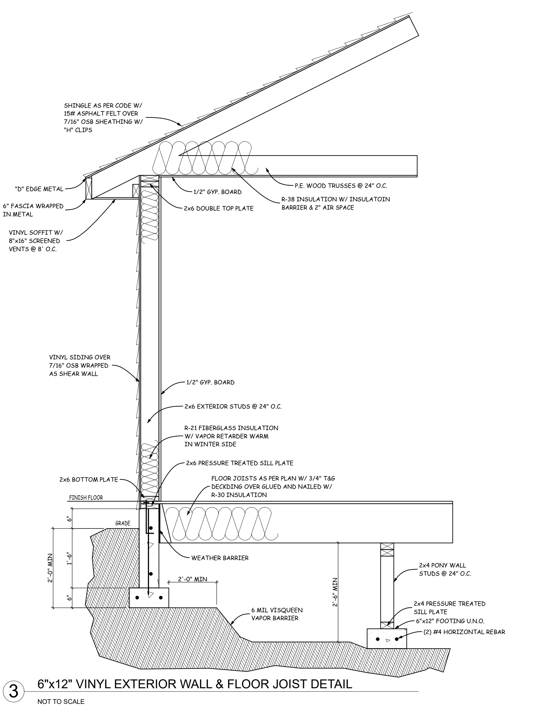
3 6"x12" VINYL EXTERIOR WALL & FLOOR JOIST DETAIL NOT TO SCALE
